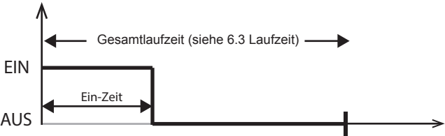
Fig. 16: Timer I/O operating mode
