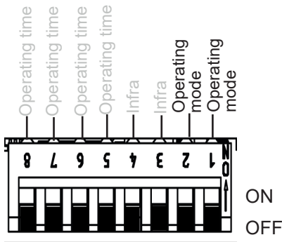
Fig. 9: Operating mode
