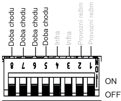
Obr. 11: Doba chodu
