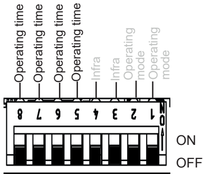
Fig. 11: Operating time
