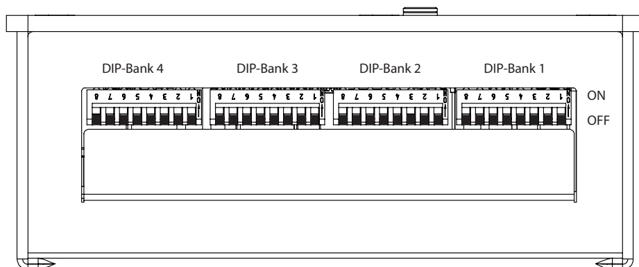
EN Fig. 8: Function selection switch - Standard setting
