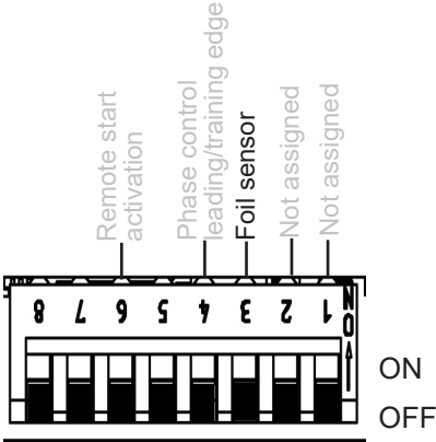
Fig. 12: Foil sensor
